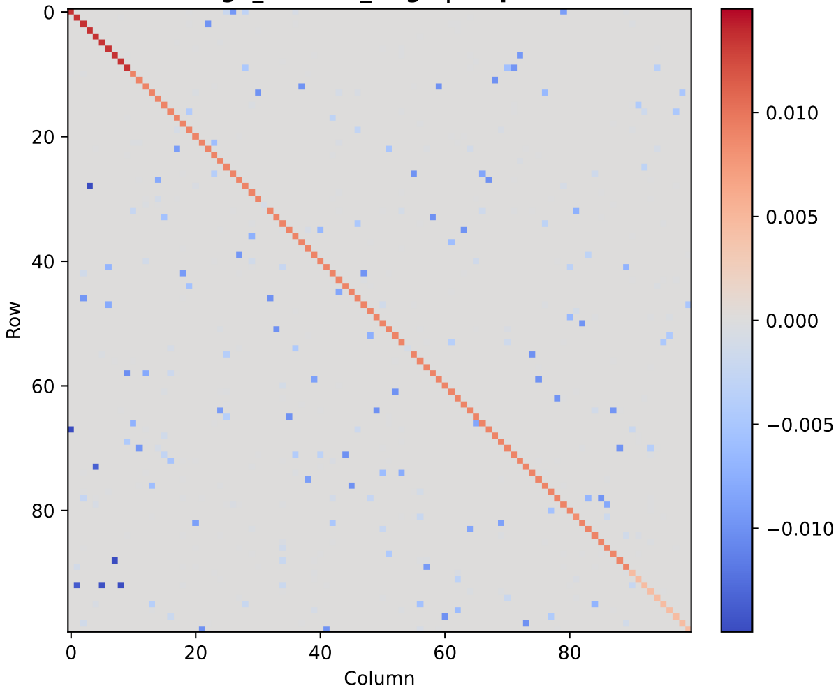
gd_random_large | step 6
